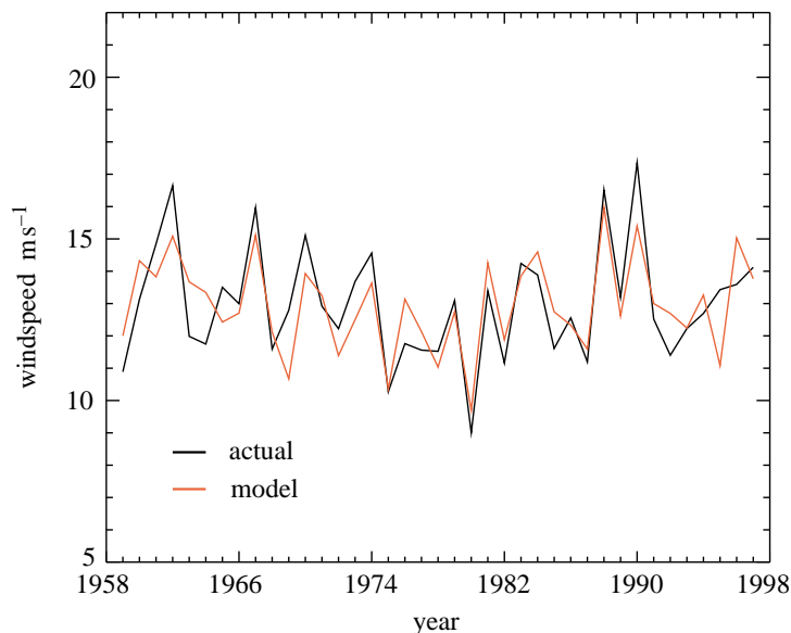
Figure 13. Comparison of model prediction and actual values for top 5% of February storminess in southeastern and eastern England 1959–1997 at 10 m. All model predictions are based on August climate data. The correlation between the two time-series is 0.80 and the model explains 63% of the variance in the observations. (From unpublished work by Steven George and Mark Saunders.)
