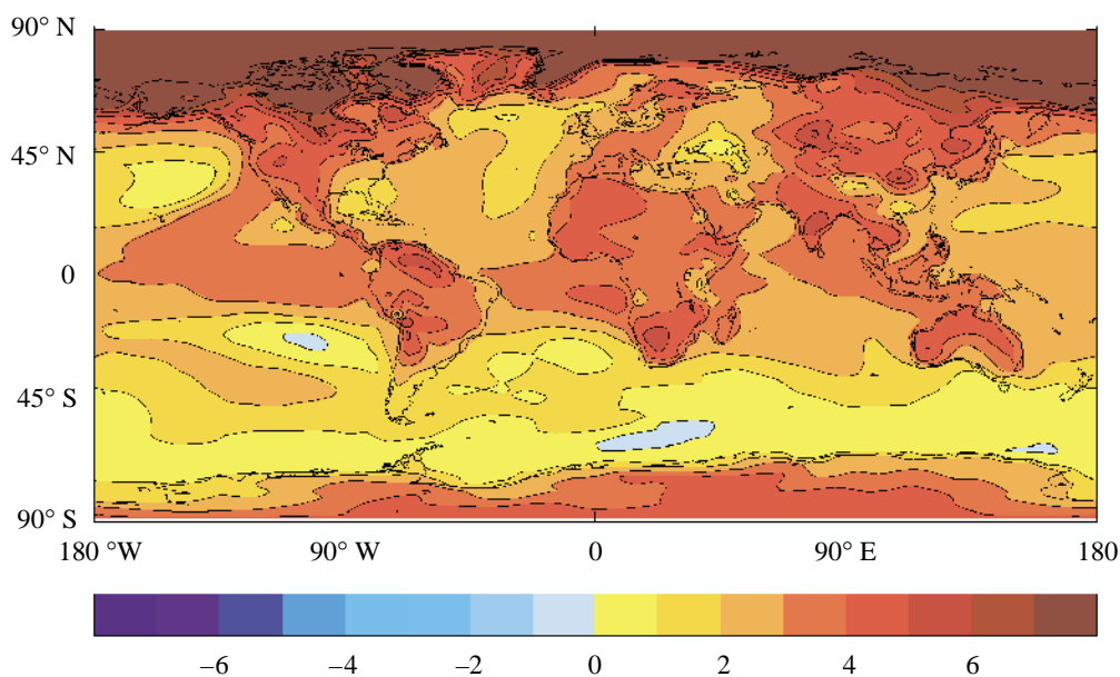
Figure 7. Change in surface temperature ( ^{\circ}\text{C} ) predicted by a climate model between 1990 and 2090 due to changes in greenhouse gases and aerosols. The figure is for Northern Hemisphere winter months. (Figure courtesy of the Hadley Centre for Climate Prediction and Research, Bracknell, UK.)
